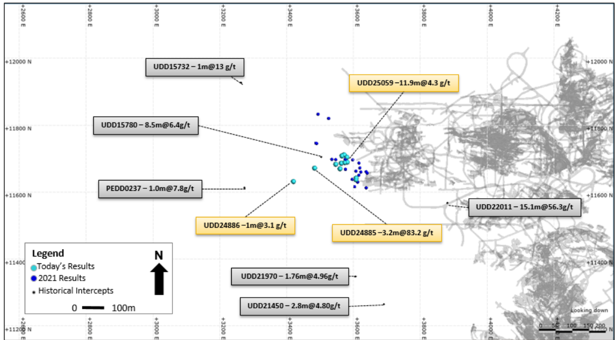
Figure 2: Significant Intercepts and Drill Hole Locations for Western Mining Front Extension Areas during Fourth Quarter 2021 (Plan View)
