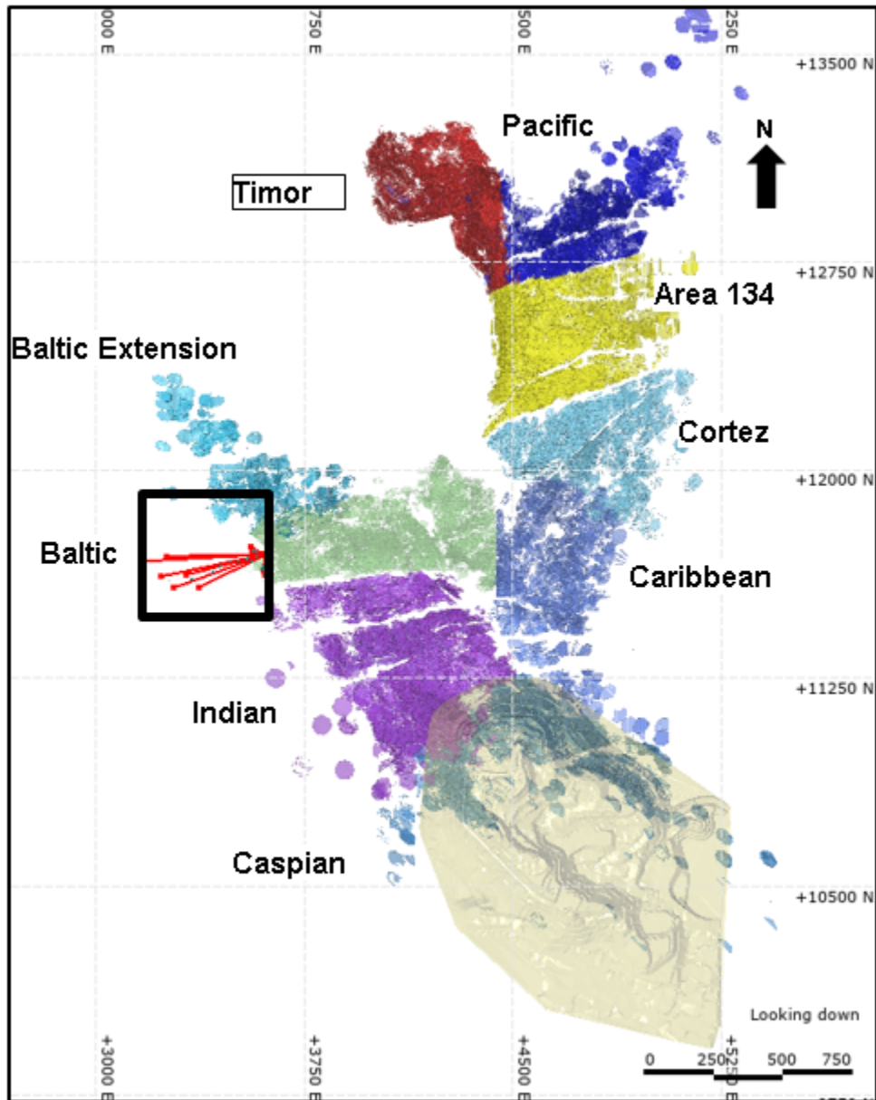
Figure 1: Mineralized Zones at Plutonic Underground with Q4, 2021 Drill Hole Locations (Plan View)
