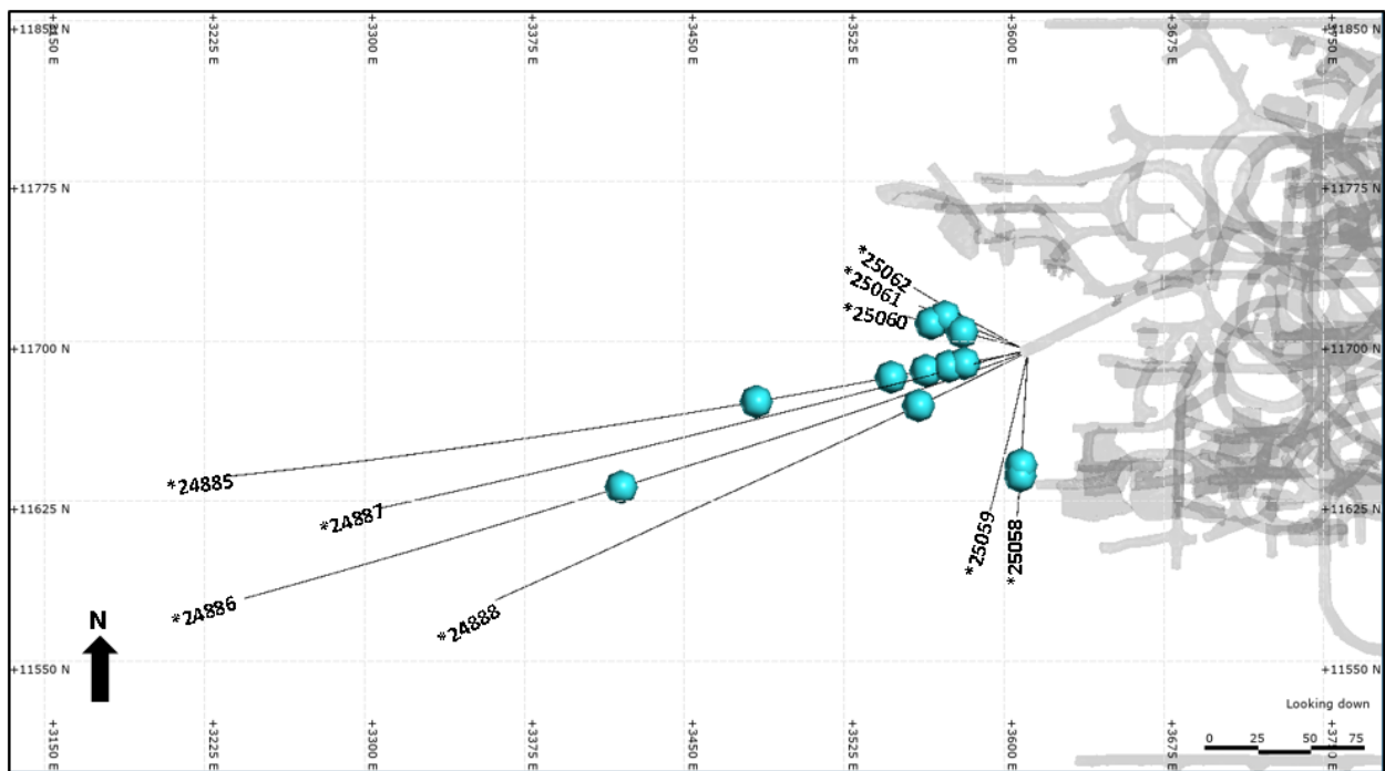
Figure 3: Plan view of Baltic Western Front Extension Significant Intercept Locations (* = UDD)
